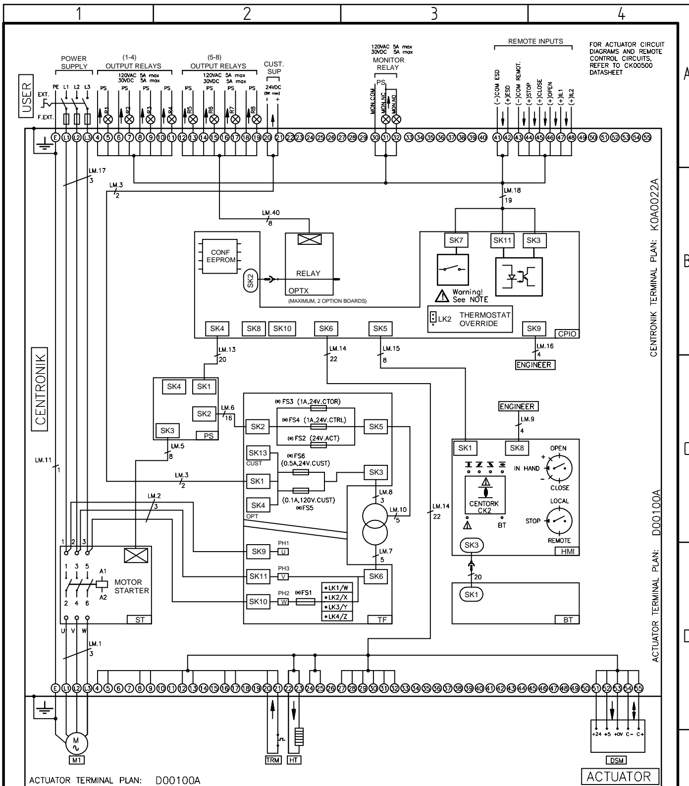
ACTUATOR TERMINAL PLAN: D00100A
